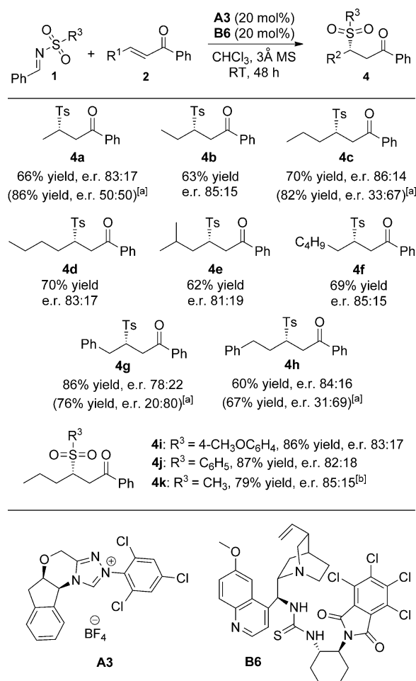
Scheme 3. Examples of the sulfonation of aliphatic enones (see the Supporting Information for detailed reaction conditions). [a] Yields and enantiomeric ratios given in the parenthesis are for reactions carried out under the conditions described in Table 1, entry 11. [b] The reaction was carried out without molecular sieves (MS). Ts = p -toluenesulfonyl.
